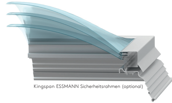
Kingspan ESSMANN Lichtkuppel classic
