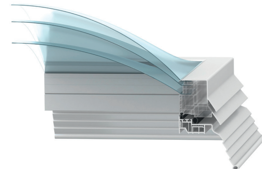
Kingspan ESSMANN Lichtkuppel neo plus
